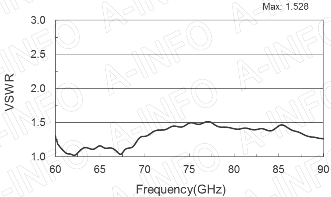
Port V_VSWR
